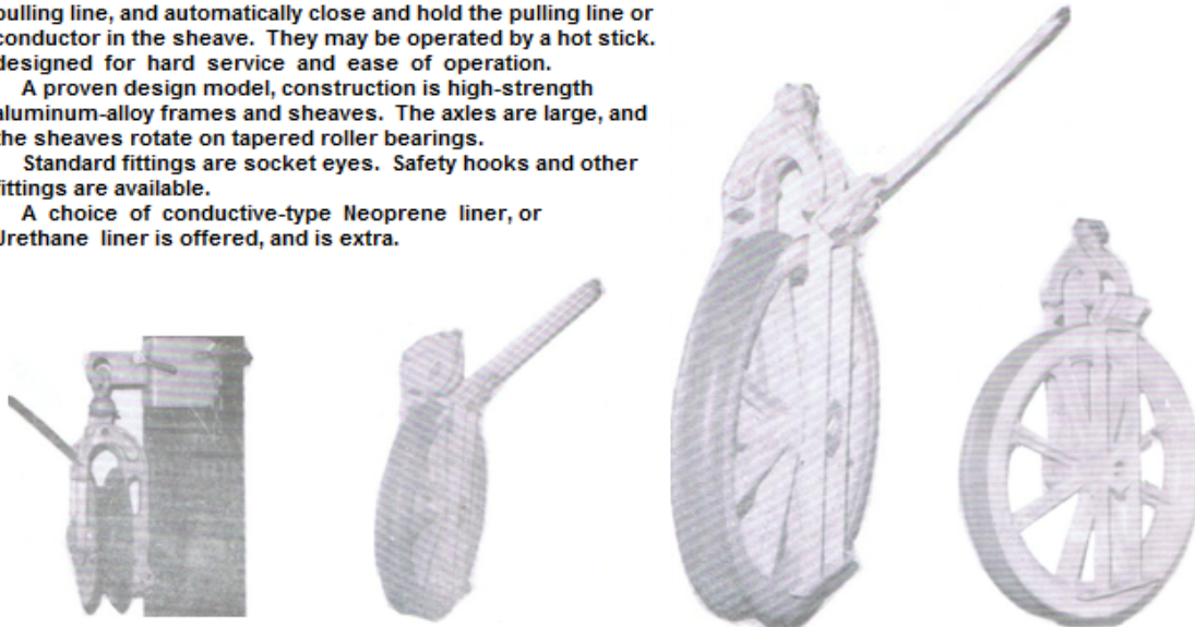
BRACKET NO. 12 BLOCK MAY BE ATTACHED TO POLE OR TOWER FOR STATIC WIRE WITH THIS BRACKET.
