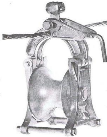
BLOCK CLAMPED WITH MESSENGER CABLE CLAMP
